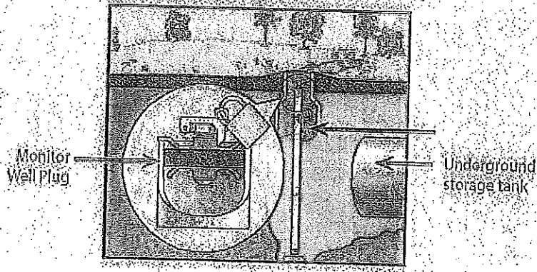
Monitor-Well Plug Installed
